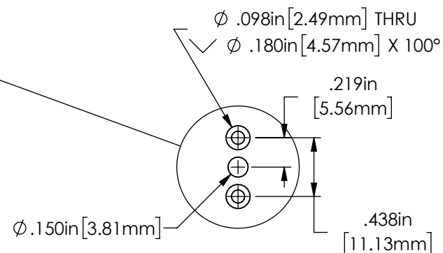
4 PLACES HOLE DETAIL FOR MS21069L06 NUTPLATE SCALE 1 : 1 (DO NOT SCALE DRAWING)
